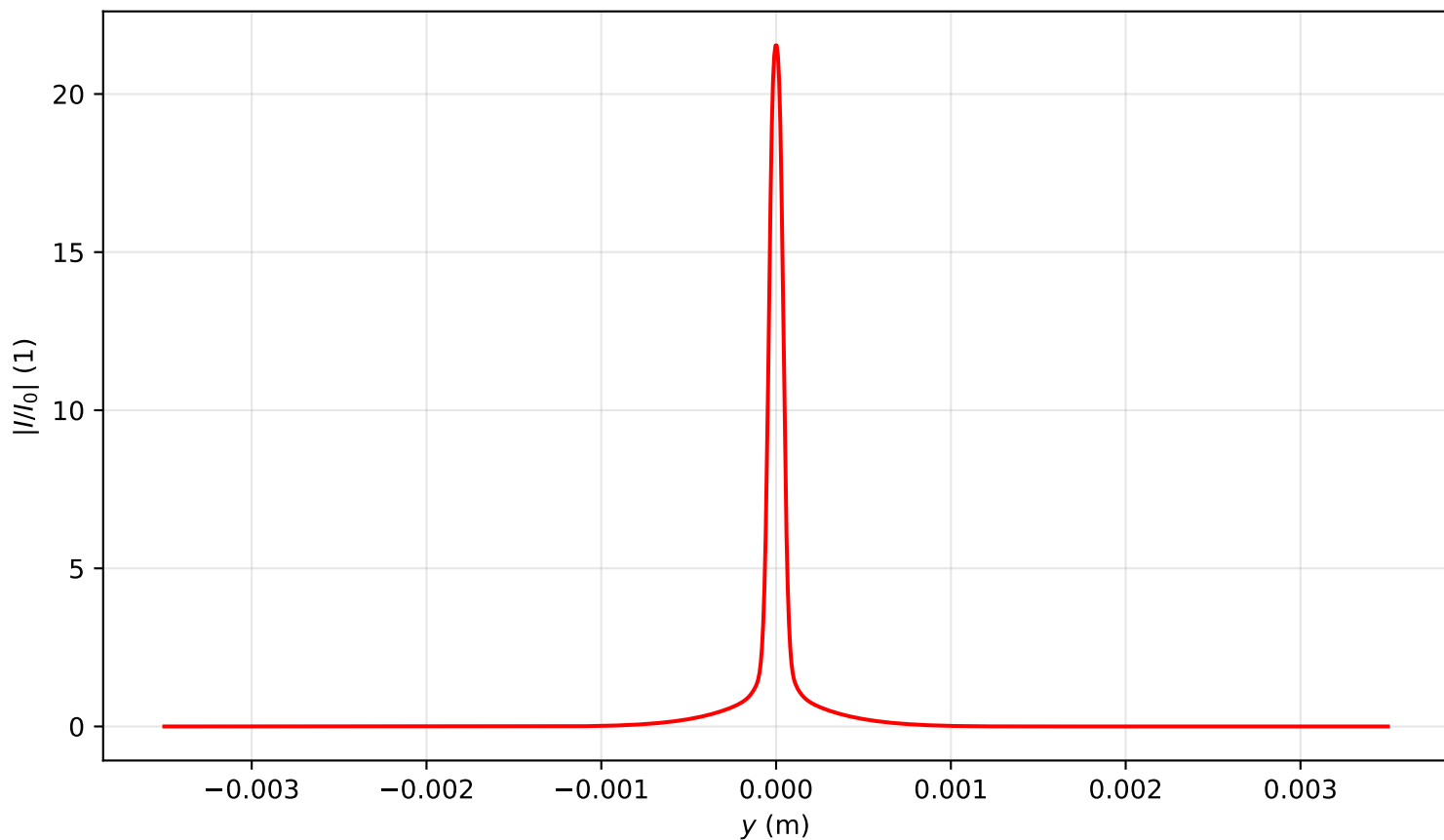
Intensity profile I(x=0, y, z=0.478)/I_0 , P_{in}=5.0P_{cr} , artificial time
